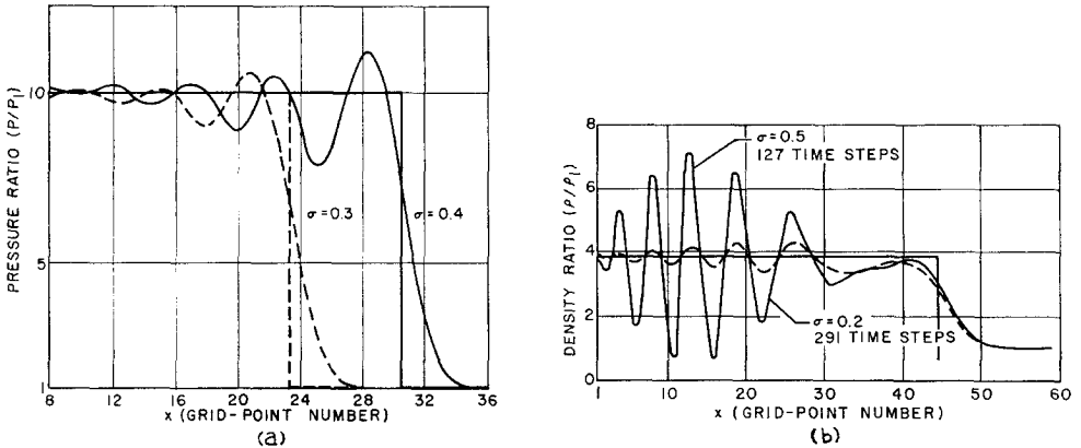
FIG. 4. Profiles for one-dimensional passage as given by Landshoff's method. (a) Pressure profile: \alpha = 2.0 , \sigma \approx 0.3, 0.4 ; (b) density profile: \alpha \approx 3.5 .
