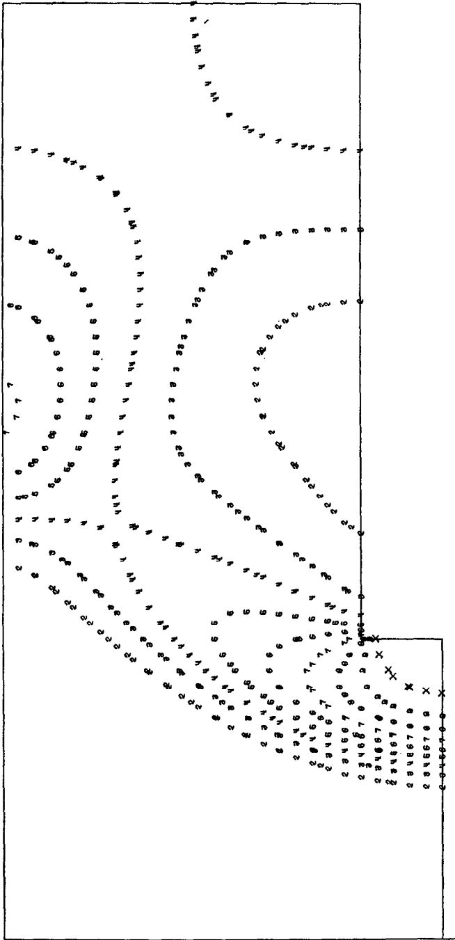
FIG. 9. Isobars ( P/P_1 ) for two-dimensional step as given by Lax's method: \sigma = 0.7 , n = 850 , n\Delta t = 147.5 \Delta x/c_1 ( x = 10 , * = 11 , \Delta = 12 ).
