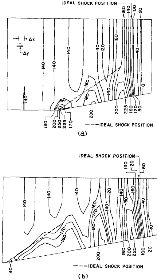
FIG. 13. Passage of a Mach-11 shock wave over an 11.5-degree half-angle cone at zero angle of attack. (a) Blunted tip; (b) sharp tip.
